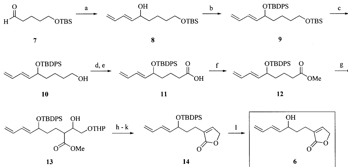
Scheme 1. Reagents and conditions: (a) ( E )- n\text{Bu}_3\text{SnCH}=\text{CHCH}=\text{CH}_2 , n\text{BuLi} , THF, -78^\circ\text{C} , 93%; (b) TBDPSCI, Imid, DMF, room temp., 100%; (c) PPTS, EtOH, room temp., 95%; (d) \text{SO}_3\cdot\text{py} , DMSO, \text{Et}_3\text{N} , \text{CH}_2\text{Cl}_2 , 0^\circ\text{C} ; (e) PDC, DMF, room temp., 82% in two steps; (f) \text{K}_2\text{CO}_3 , MeI, DMF, 0^\circ\text{C} , 99%; (g) LDA, \text{THPOCH}_2\text{CHO} , THF, -78^\circ\text{C} , 95%; (h) PPTS, MeOH, room temp.; (i) \text{Et}_3\text{N} , MeOH, room temp.; (j) \text{Ac}_2\text{O} , py, room temp.; (k) DBU, PhMe, 0^\circ\text{C} , 87% in four steps; (l) TBAF, AcOH, THF, room temp., 92%.
