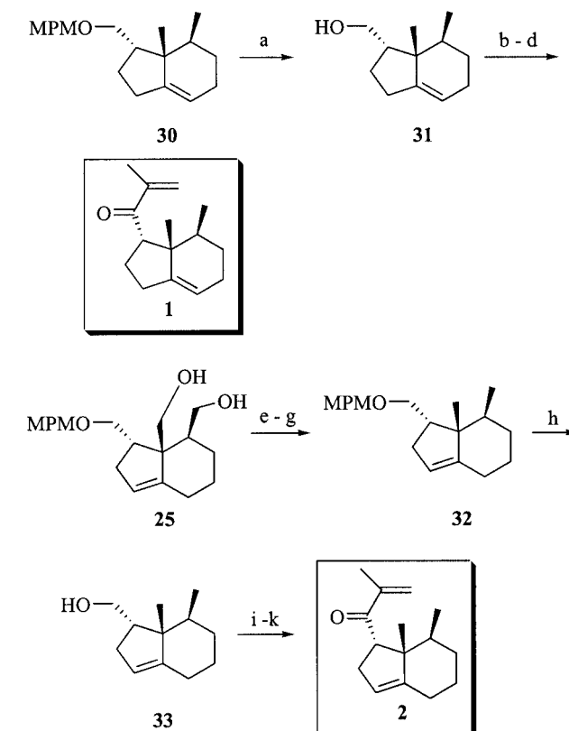
Scheme 5. Reagents and conditions: (a) DDQ, CH 2 Cl 2 , H 2 O, 0 °C, 92%; (b) IBX, DMSO, THF, room temp.; (c) CH 2 =C(Me)MgBr, THF, 0 °C; (d) IBX, DMSO, THF, room temp., 75% in three steps; (e) MsCl, py, room temp.; (f) Na 2 S·9H 2 O, DMF, 50 °C; (g) Raney Ni W-4, THF, room temp., 60% in three steps; (h) DDQ, CH 2 Cl 2 , H 2 O, 0 °C, 85%; (i) IBX, DMSO, THF, room temp.; (j) CH 2 =C(Me)MgBr, THF, 0 °C; (k) IBX, DMSO, THF, room temp., 73% in three steps.
