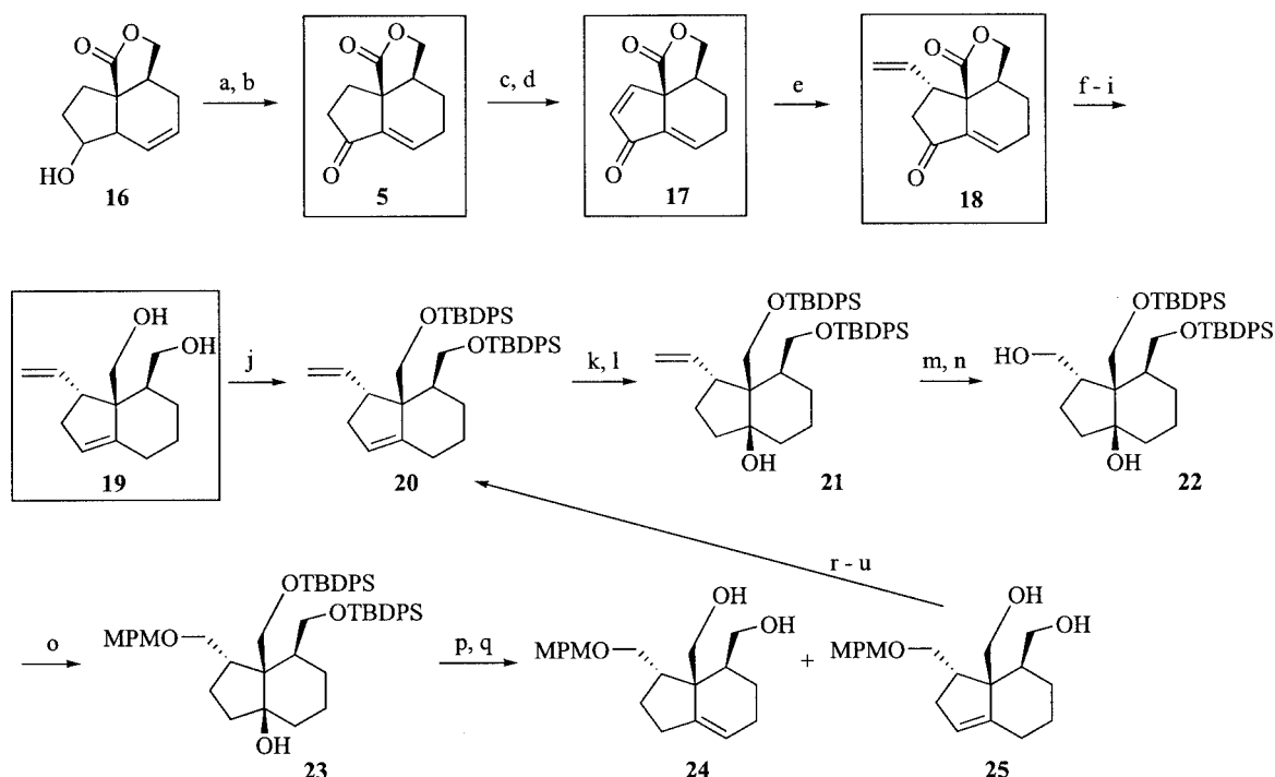
Scheme 3. Reagents and conditions: (a) TFAA, DMSO, Et 3 N, CH 2 Cl 2 , –60 °C; (b) DBU, PhMe, 0 °C, 87% in two steps; (c) TMSOTf, Et 3 N, CH 2 Cl 2 , 0 °C; (d) Pd(OAc) 2 , CH 3 CN, room temp., 98% in two steps; (e) CH 2 =CHMgBr, CuI, THF, –78 °C, 75%; (f) NaBH 4 , MeOH, 0 °C; (g) MsCl, py, room temp.; (h) AcOK, DMF, H 2 O, 80 °C; (i) DIBAL-H, CH 2 Cl 2 , 0 °C, 75% in four steps; (j) TBDPSCl, Imid, DMF, 0 °C, 97%; (k) m CPBA, NaH 2 PO 4 , CH 2 Cl 2 , –20 °C; (l) LiEt 3 BH, THF, room temp., 74% in two steps; (m) OsO 4 , Me 3 NO, acetone, H 2 O, room temp.; then NaIO 4 , NaH 2 PO 4 , room temp.; (n) NaBH 4 , MeOH, 0 °C, 58% in two steps; (o) MPMCl, NaH, n Bu 4 NI, DMF, 0 °C, 70%; (p) SOCl 2 , py, –30 °C; (q) TBAF, THF, 50 °C, 94% ( 24 : 18%, 25 : 76%) in two steps; (r) TBDPSCl, Imid, DMF, 0 °C; (s) DDQ, CH 2 Cl 2 , H 2 O, 0 °C; (t) IBX, DMSO, THF, room temp.; (u) Ph 3 PCH 3 Br, NaHMDS, THF, –40 °C, 65% in four steps.
